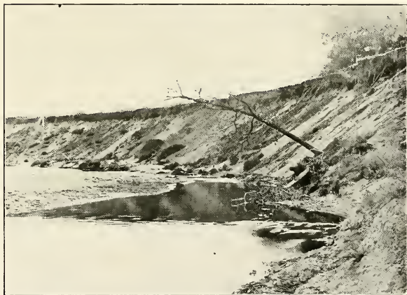
B. Crow Creek, west of Henry, widening its valley by lateral erosion. (Photo by Crane.)
